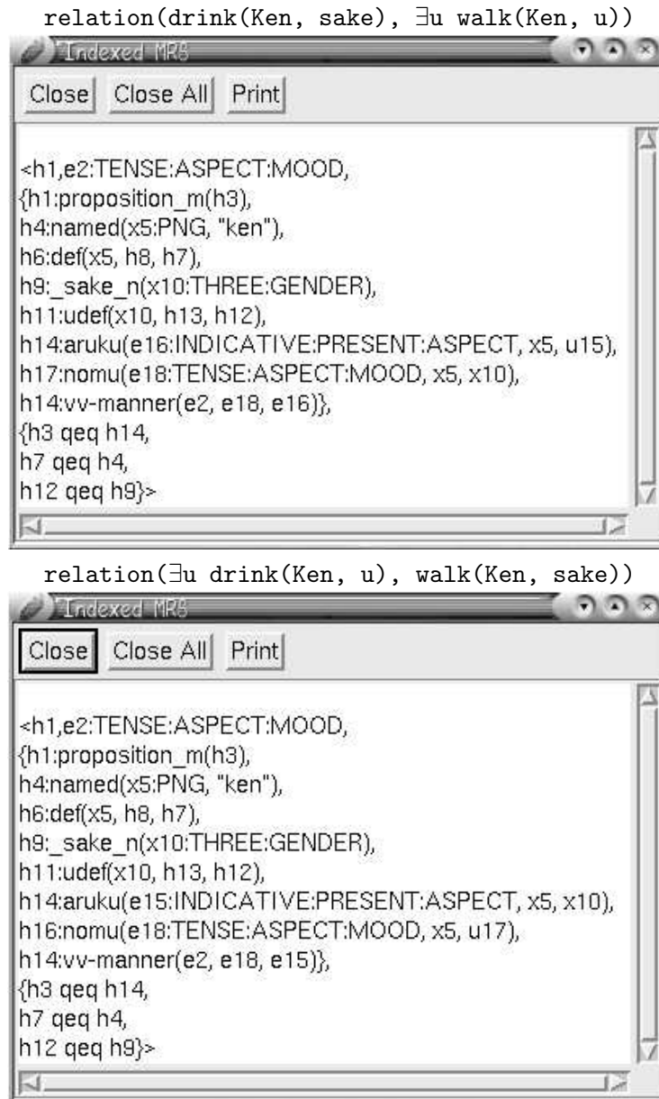
Figure 19: The JACY output of Ken-ga sake-o nomi-aruku : semantics
